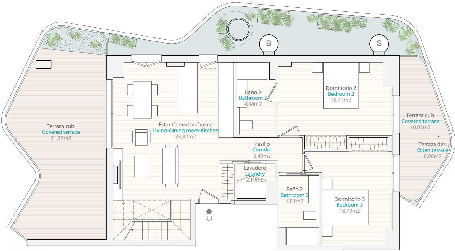
PLANTA 6 | Floor 6
