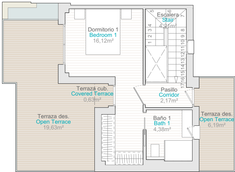
Planta 1 | Floor 1
